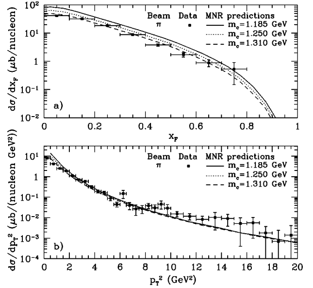
FIG. 3. Comparison of differential cross sections for (D^+, D^-, D^0, \bar{D}^0) production, calculated using MNR at different m_c values, with WA92 data for \pi N [9]: (a) d\sigma/dx_F , (b) d\sigma/dp_T^2 ( x_F > 0 ) (PDF: MRS R1).
