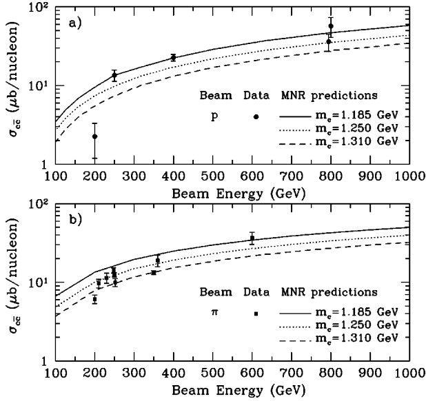
FIG. 1. Comparison of experimental data for \sigma_{cc^-} with MNR predictions for different m_c values: (a) in pN collisions (Ref. [10], Table I), (b) in \pi N collisions (Ref. [10], Table II) (PDF: MRS R1).
