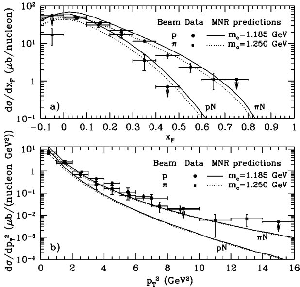
FIG. 2. Comparison of differential cross sections for (D^+, D^-, D^0, \bar{D}^0, D_S^+, \text{ and } D_S^-) production, calculated using MNR at different m_c values, with E769 data for pN and \pi N [8]: (a) d\sigma/dx_F , (b) d\sigma/dp_T^2 ( x_F > 0 ) (PDF: MRS R1).
